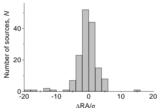
Figure 2: The distribution of \Delta RA and \Delta RA/\sigma for the Texas survey. The parameters of the gaussian curve (upper panel) are M = -0.038 s, sd = 0.156 s.
